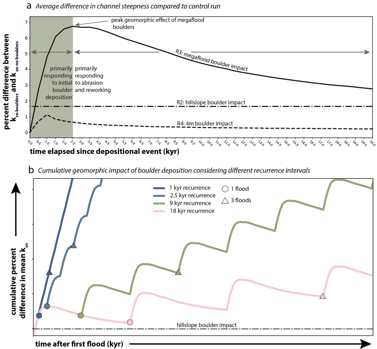
Figure 3. (a) Average local percent change in k_{sn} between R2, R3, and R4 with respect to the baseline at each time-step of the model run as a function of time elapsed after the megaflood depositional event (b) Schematic of cumulative geomorphic impact due to the addition of megaflood boulders from sequences of many floods with four different recurrence intervals: 1, 2.5, 9, and 18 kyr. The dashed line is the same dashed line from (a)—the equilibrium effect of a landscape that experiences hillslope-derived boulder deposition.
